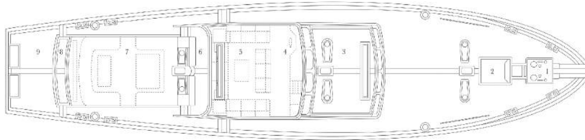
1. Windlass 2. Crew Entrance 3. Dining-Saloon 4. Bridge 5. Main Saloon 6. Fly-Bridge 7. Cockpit 8. Storage 9. Aft Platform
