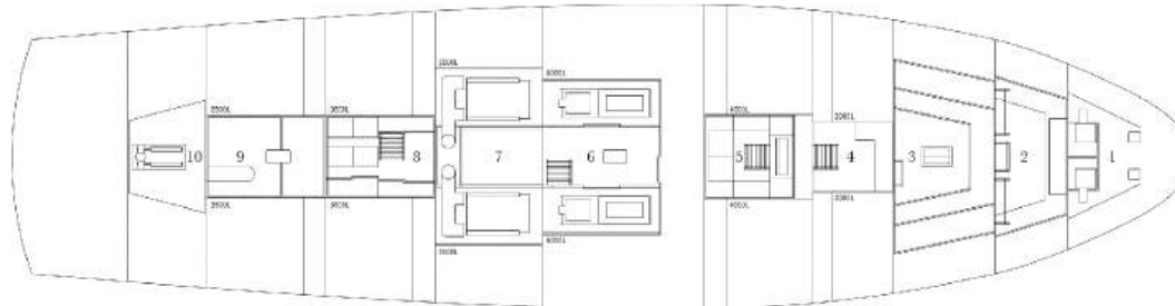
1. Fore Peak 2. Forepeak 3. Dry Stores 4. Workshop 5. Laundry 6. Upper Engine Room 7. Lower Engine Room 8. Pump Room 9. Spares/Stores 10. Steering Rudder Assembly
